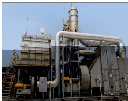
VOC Treatment System
